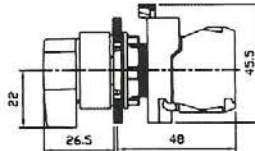
ISS-90 ILLUMINATED (90° - 2 Position)
