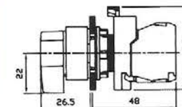
NLS-22 ILLUMINATED (90° - 2 Position)
