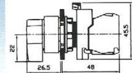
NLSS-22 ILLUMINATED (45° - 3 Position)
